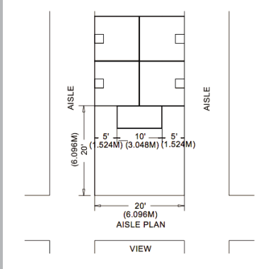
PENINSULA BOOTH PLAN VIEW
