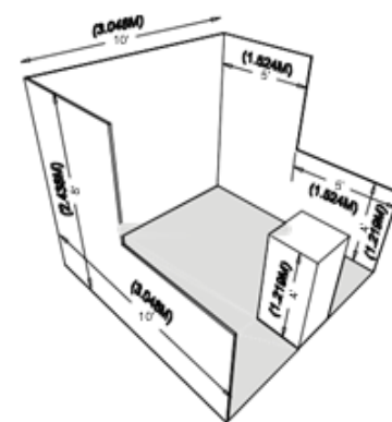
LINEAR BOOTH 3D VIEW
