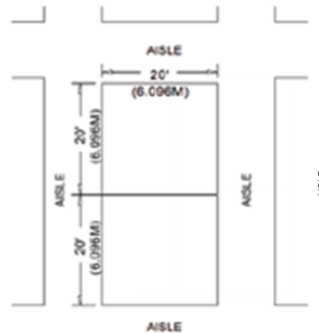
SPLIT ISLAND BOOTH PLAN VIEW
