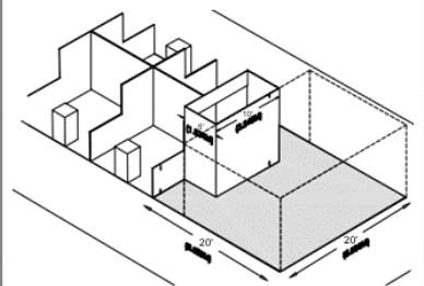
PENINSULA BOOTH 3D VIEW
